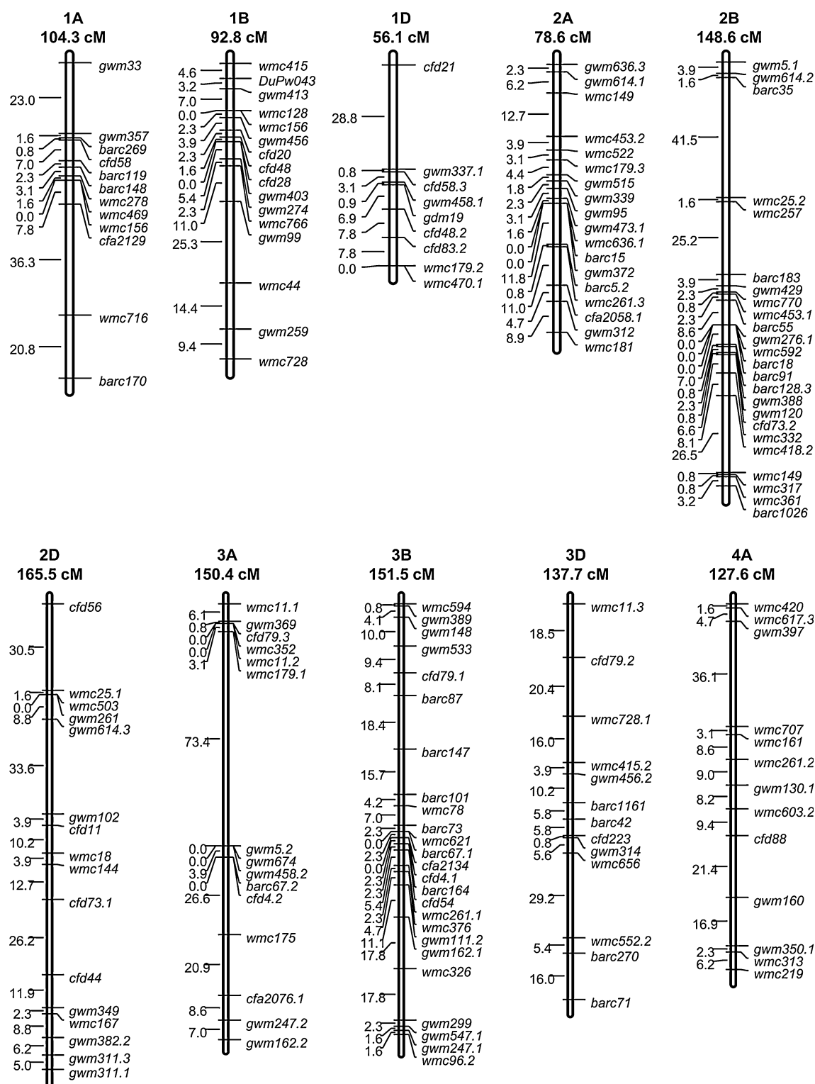
Fig. 2 Genetic linkage maps constructed in the Grandin × PI 277012 derived DH population. The positions of marker loci are shown to the right of the linkage groups and centiMorgan (cM) distances between loci are shown along the left. Linkage maps were developed using the
